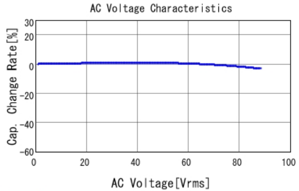
GRJ21BR72E223KWJ3 C-AC Voltage capchange, DCOV, 25
