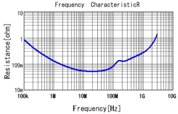
GRJ21BR72E223KWJ3 R DCOV, 25degC
