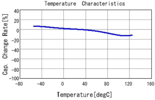
GRJ21BR72E223KWJ3 C-Temp. capchange, DCOV, AC1Vrms
