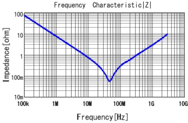
GRJ21BR72E223KWJ3 |Z| DCOV, 25degC
