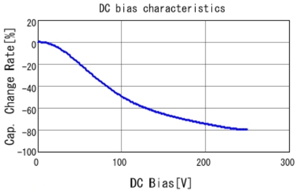
GRJ21BR72E223KWJ3 C-DC bias capchange, 25.0degC, A
