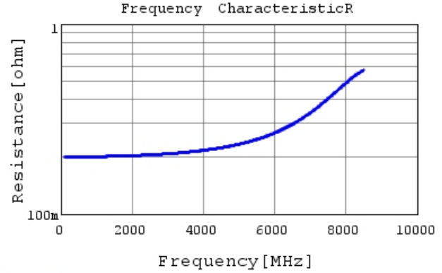
GJM1555C1H1R7BB01 R DC0V, 25degC
