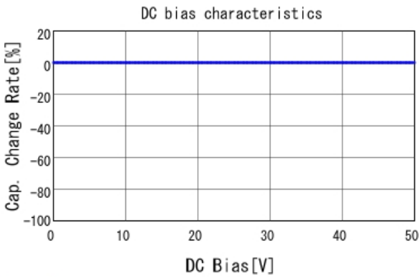
GCM1555G1H220JA16 C-DC bias capchange, 25.0degC, A
