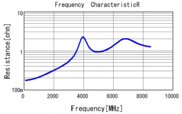
GCM1555G1H220JA16 R DCOV, 25degC
