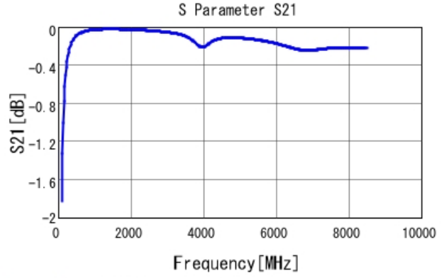
GCM1555G1H220JA16 S21 DCOV, 25degC
