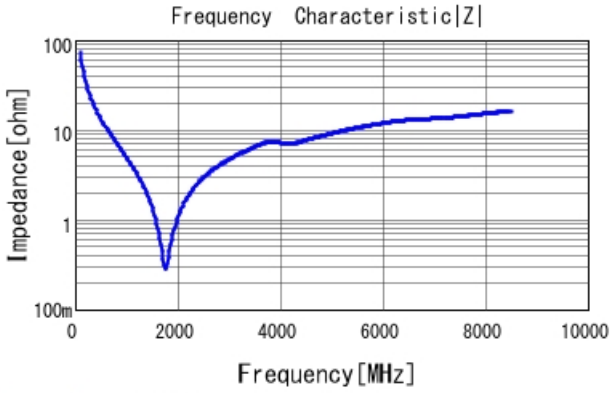
GCM1555G1H220JA16 |Z| DCOV, 25degC
