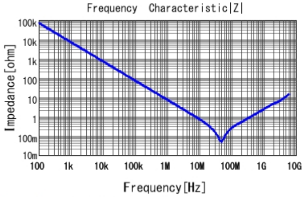
GCM188R71E223KA37 |Z| DCOV, 25degC
