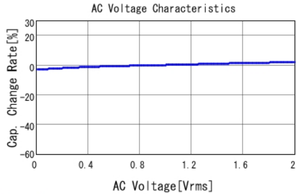
GCM188R71E223KA37 C-AC Voltage capchange, DCOV, 25
