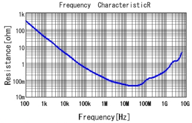
GCM188R71E223KA37 R DCOV, 25degC
