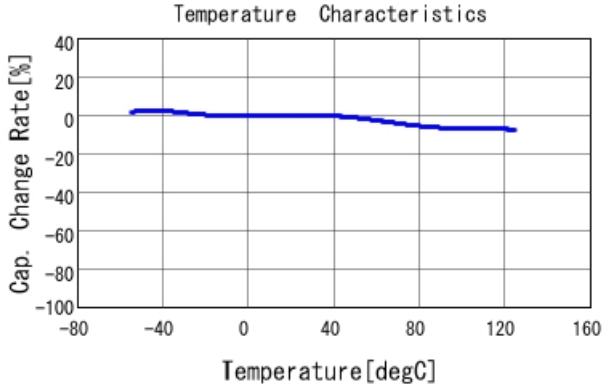
GCM188R71E223KA37 C-Temp. capchange, DC0.0V, AC1.C
