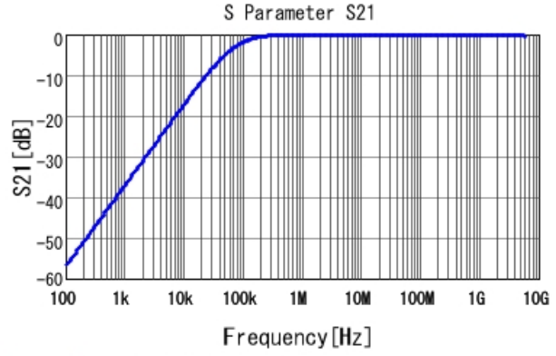
GCM188R71E223KA37 S21 DC0V, 25degC
