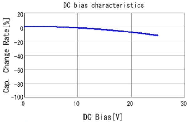
GCM188R71E223KA37 C-DC bias capchange, 25.0degC, A
