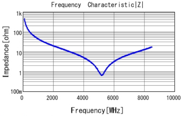
GRM0335C1H3R5BA01 |Z| DCOV, 25degC
