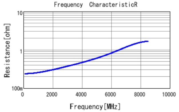
GRM0335C1H3R5BA01 R DCOV, 25degC
