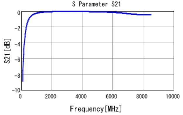
GRM1555C1H6R1DA01 S21 DCOV, 25degC
