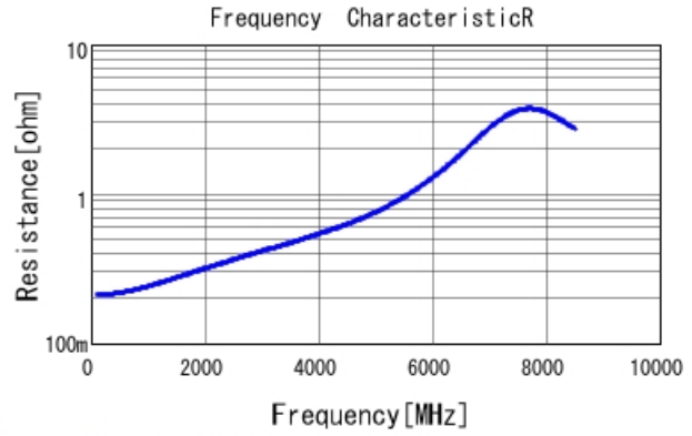
GRM1555C1H6R1DA01 R DCOV, 25degC
