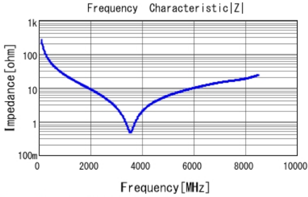
GRM1555C1H6R1DA01 |Z| DCOV, 25degC
