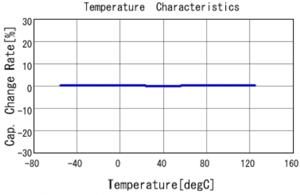
GRM1555C1H6R1DA01 C-Temp. capchange, DCOV, AC1Vrms
