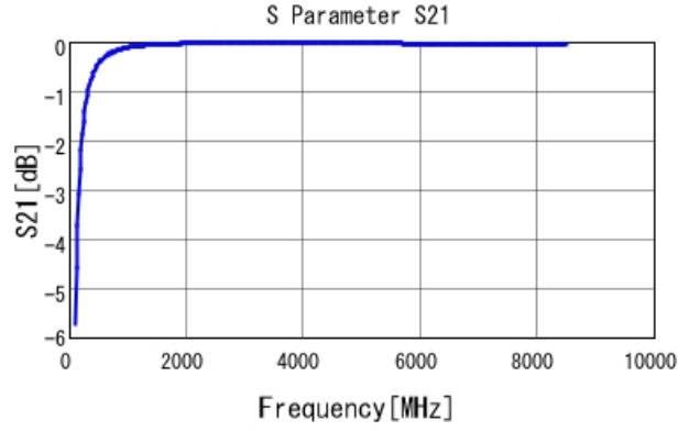
GRM0225C1E9R6WA03 S21 DCOV, 25degC
