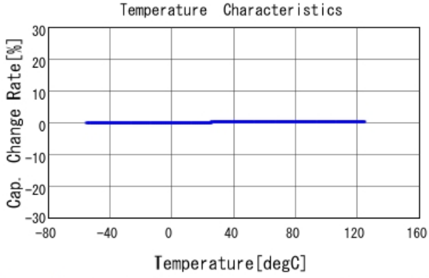
GRM0225C1E9R6WA03 C-Temp. capchange, DCOV, AC1Vrms
