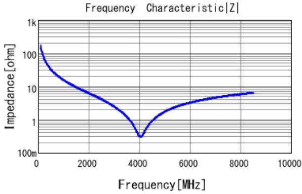
GRM0225C1E9R6WA03 |Z| DCOV, 25degC
