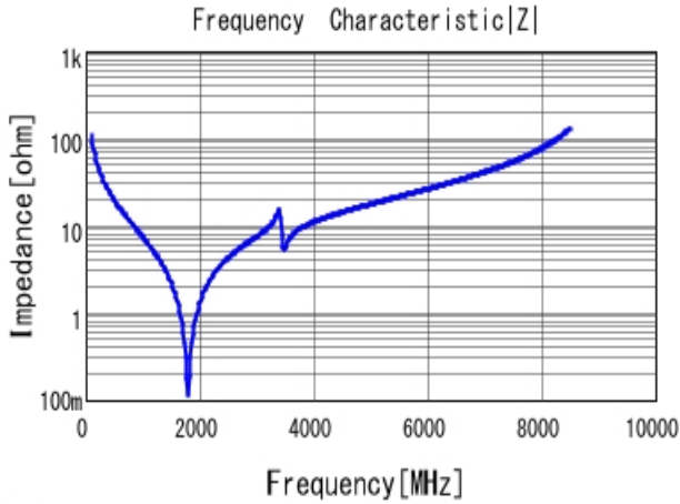
■ GQM1885C1H150GB01 |Z| DCOV, 25degC
