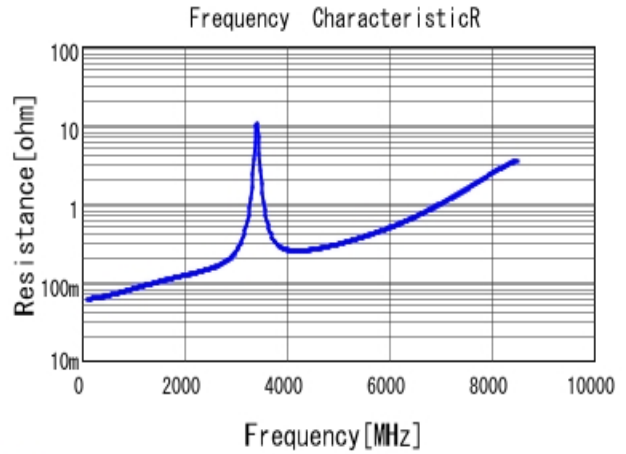
■ GQM1885C1H150GB01 R DCOV, 25degC
