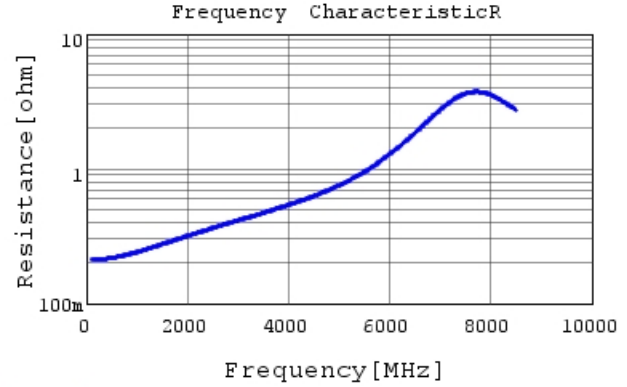
GRT1555C1H6R0DA02 R DCOV, 25degC
