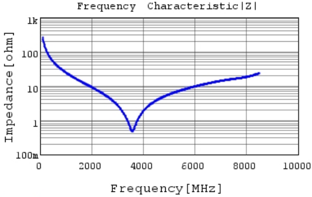
GRT1555C1H6R0DA02 |Z| DCOV, 25degC
