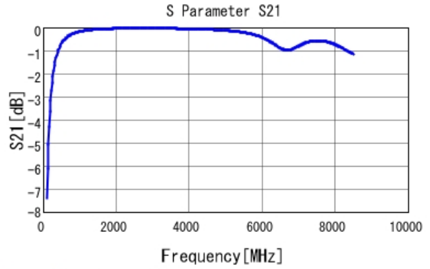
GRM1555C2A7R5WA01 S21 DC0V, 25degC
