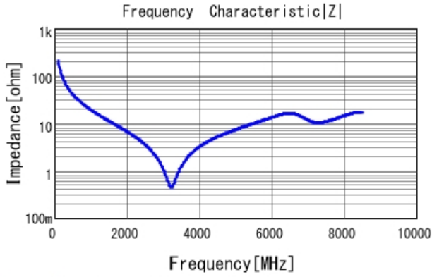
GRM1555C2A7R5WA01 |Z| DCOV, 25degC
