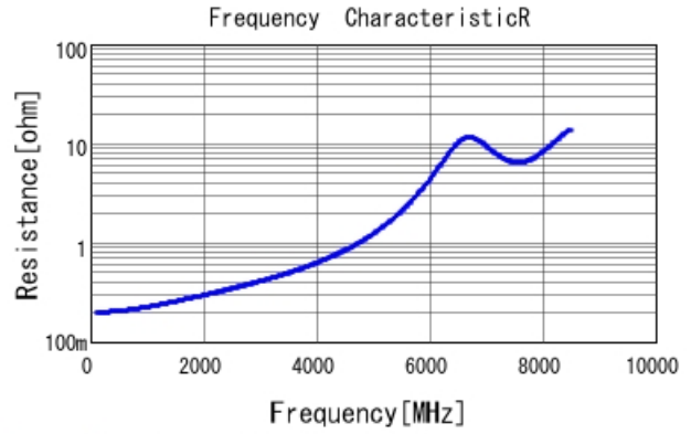
GRM1555C2A7R5WA01 R DCOV, 25degC
