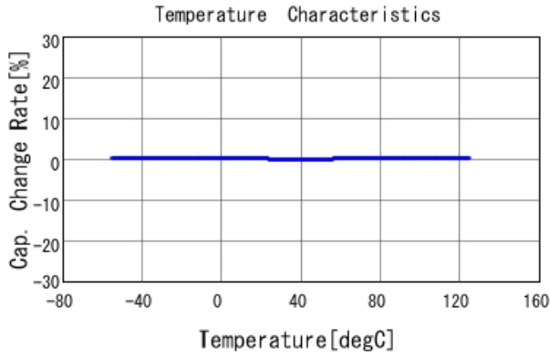
GRM1555C2A7R5WA01 C-Temp. capchange, DC0V, AC1Vrms
