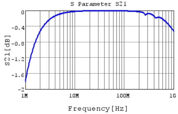
RDE7U2J222J2M1H03A S21 DCOV, 25degC
