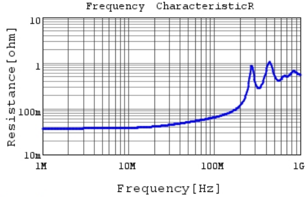
RDE7U2J222J2M1H03A R DC0V, 25degC
