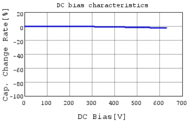
RDE7U2J222J2M1H03A C-DC bias capchange, 25.0
