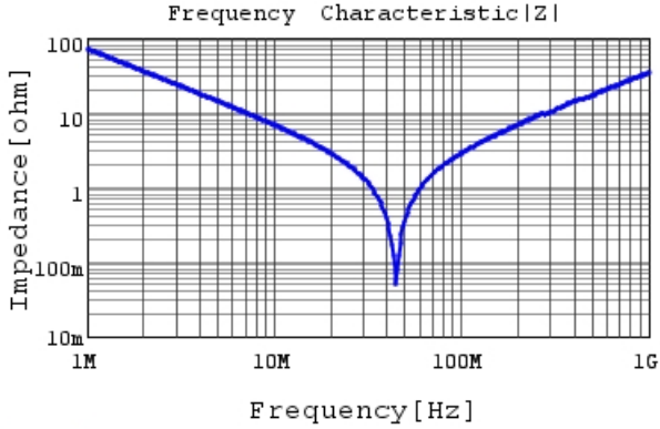
RDE7U2J222J2M1H03A |Z| DC0V, 25degC
