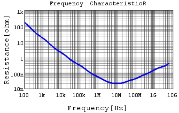
GRM033R61C224ME14 R DCOV, 25degC
