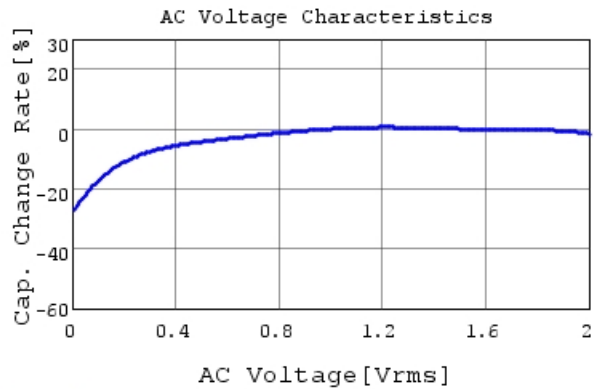
GRM033R61C224ME14 C-AC Voltage capchange, Dc
