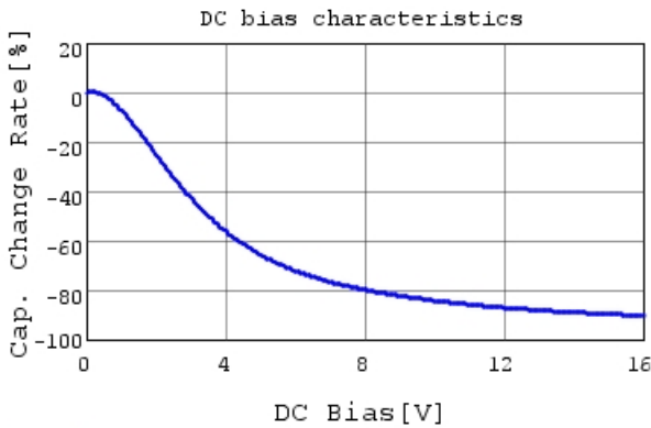
GRM033R61C224ME14 C-DC bias capchange, 25.0c
