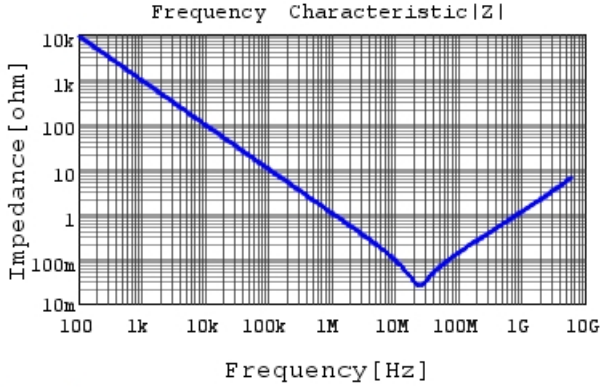
GRM033R61C224ME14 |Z| DCOV, 25degC
