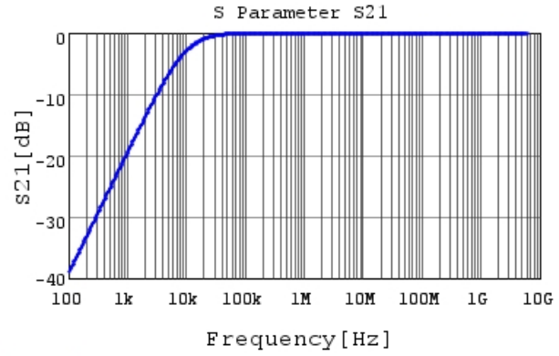
GRM033R61C224ME14 S21 DC0V, 25degC
