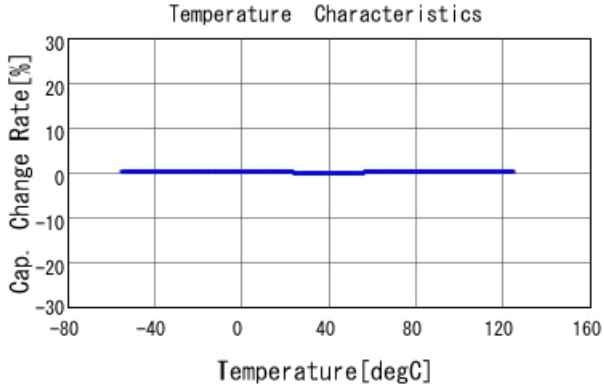
GRM1555C2A8R1BA01 C-Temp. capchange, DCOV, AC1Vrms
