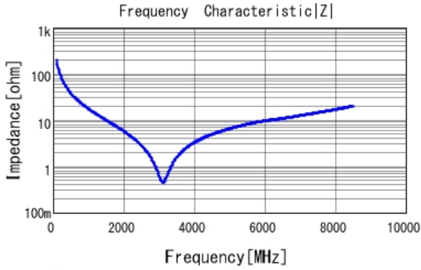
GRM1555C2A8R1BA01 |Z| DCOV, 25degC
