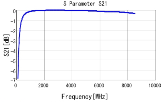
GRM1555C2A8R1BA01 S21 DCOV, 25degC
