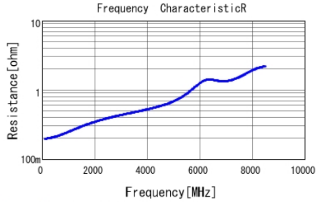
GRM1555C2A8R1BA01 R DCOV, 25degC
