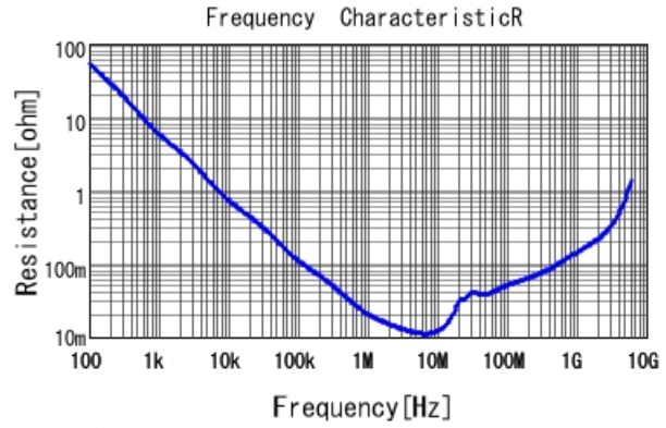
GRM188R61C684MA75 R DCOV, 25degC
