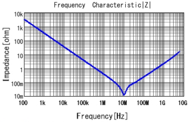
GRM188R61C684MA75 |Z| DCOV, 25degC
