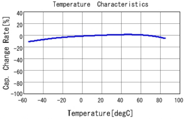
GRM188R61C684MA75 C-Temp. capchange, DC0.0V, AC1.C
