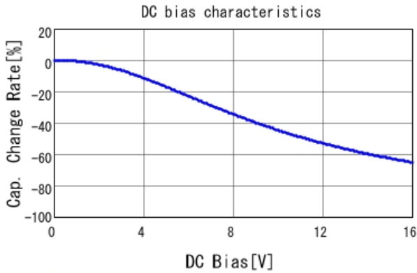
GRM188R61C684MA75 C-DC bias capchange, 25.0degC, A
