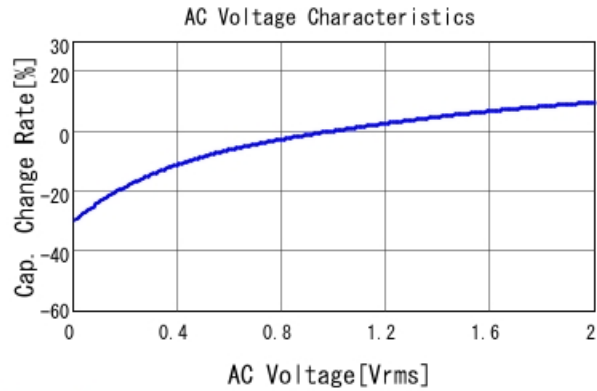
GRM188R61C684MA75 C-AC Voltage capchange, DCOV, 25
