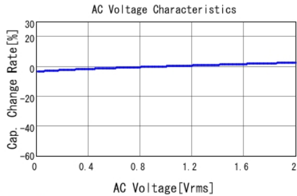
GRM55RR71H105KA01 C-AC Voltage capchange, DCOV, 25
