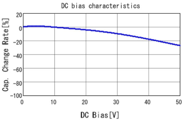
GRM55RR71H105KA01 C-DC bias capchange, 25.0degC, A
