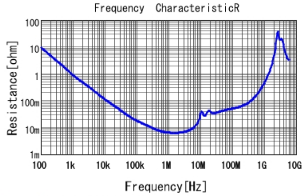
GRM55RR71H105KA01 R DCOV, 25degC
