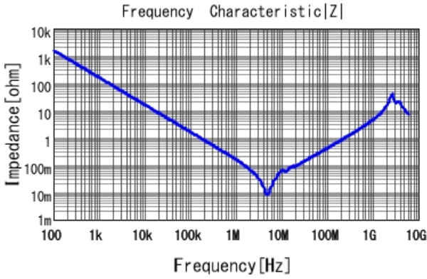
GRM55RR71H105KA01 |Z| DCOV, 25degC
