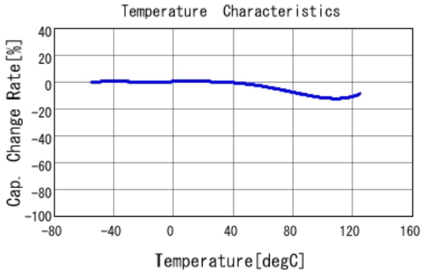
GRM55RR71H105KA01 C-Temp. capchange, DC0.0V, AC1.C
