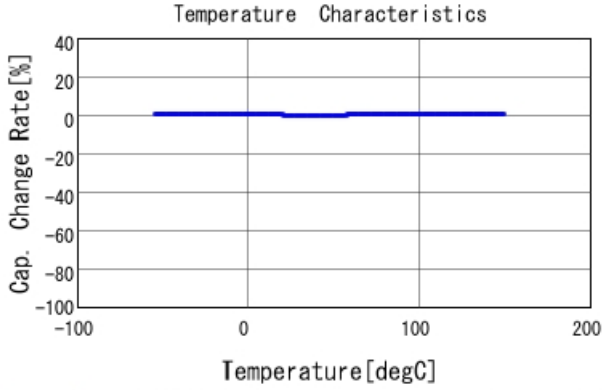
GCM1555G1H101FA16 C-Temp. capchange, DCOV, AC1Vrms
