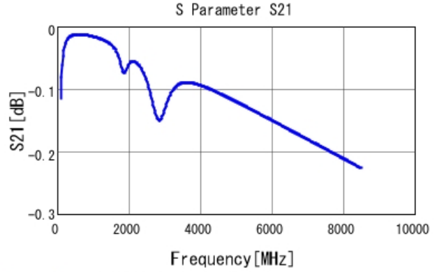
GCM1555G1H101FA16 S21 DCOV, 25degC
