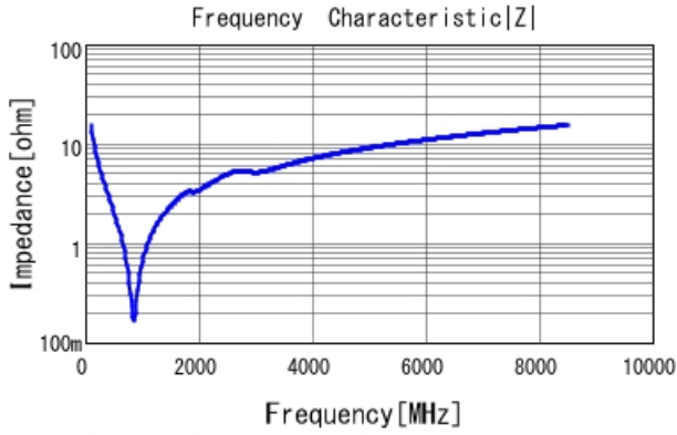
GCM1555G1H101FA16 |Z| DCOV, 25degC
