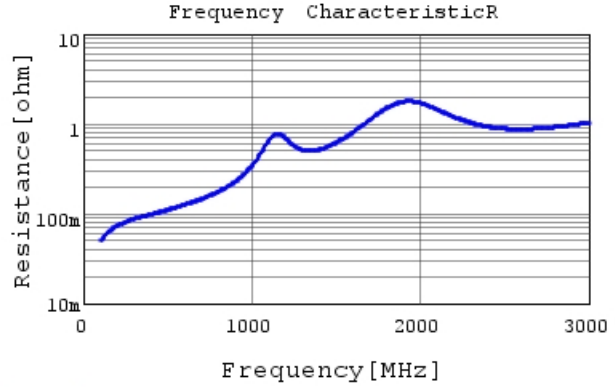
GCM21A5C2J221JX01 R DC0V, 25degC
