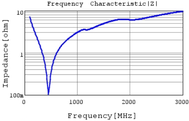
GCM21A5C2J221JX01 |Z| DC0V, 25degC
