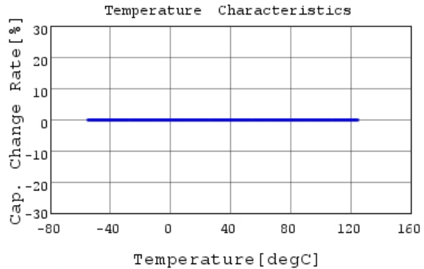
GCM21A5C2J221JX01 C-Temp. capchange, DC0V, f
