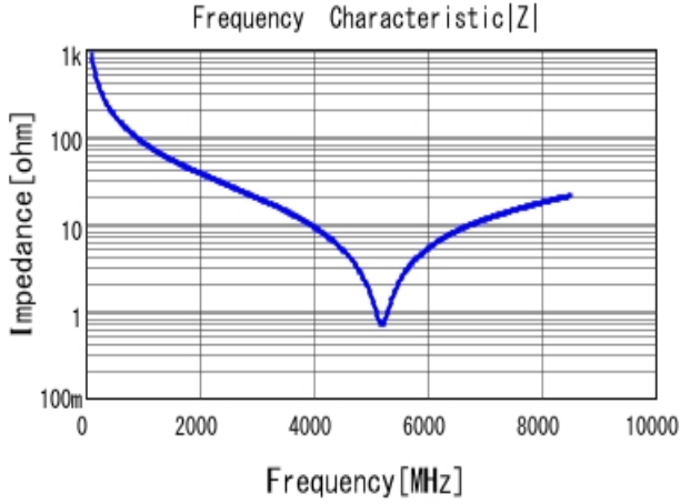
■ GRM1885C1H1R8BA01 |Z| DCOV, 25degC
