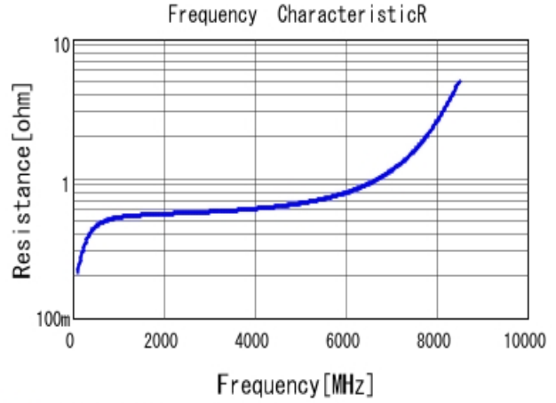
■ GRM1885C1H1R8BA01 R DCOV, 25degC
