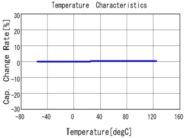
■ GRM1885C1H1R8BA01 C-Temp. capchange, DCOV, AC1Vrms
