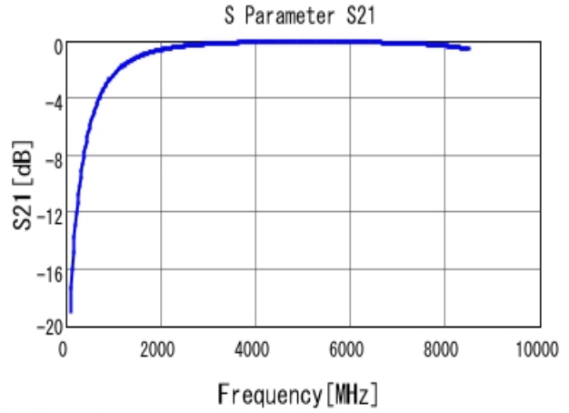
■ GRM1885C1H1R8BA01 S21 DCOV, 25degC
