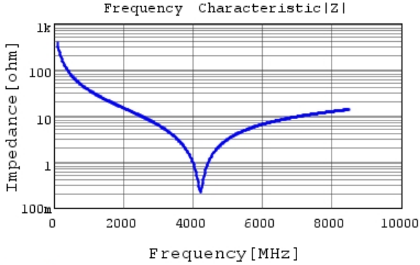
GCQ1555C1H4R2CB01 |Z| DC0V, 25degC
