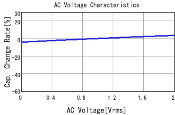
GCJ21BR71E394KA01 C-AC Voltage capchange, DCOV, 25
