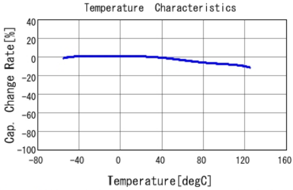
GCJ21BR71E394KA01 C-Temp. capchange, DC0.0V, AC1.C
