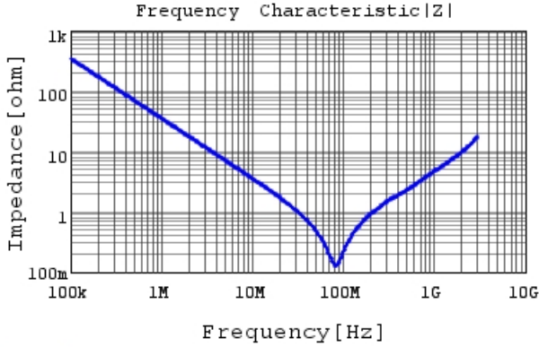
GCJ31BR73A472KXJ1 |Z| DC0V, 25degC
