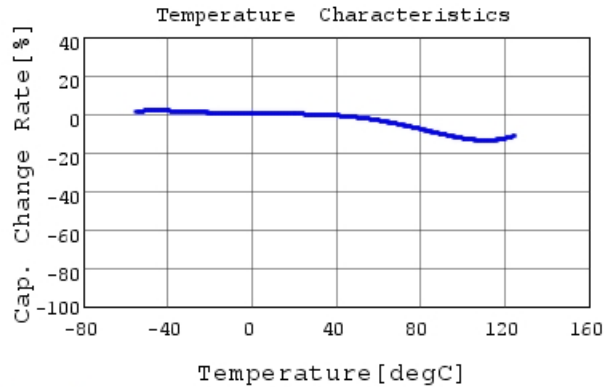
GCJ31BR73A472KXJ1 C-Temp. capchange, DC0V, 1
