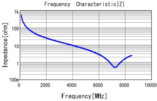
GRM0225C1E2R9CA03 |Z| DCOV, 25degC
