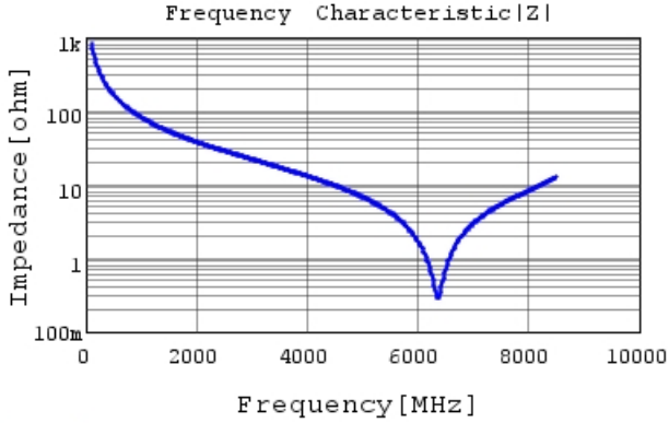
GCQ1555C1H1R9WB01 |Z| DC0V,25degC
