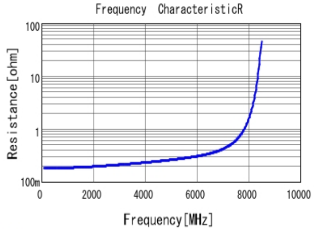
■ GQM1885C2A2R2CB01 R DCOV, 25degC
