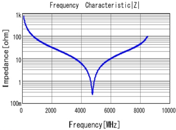
■ GQM1885C2A2R2CB01 |Z| DCOV, 25degC
