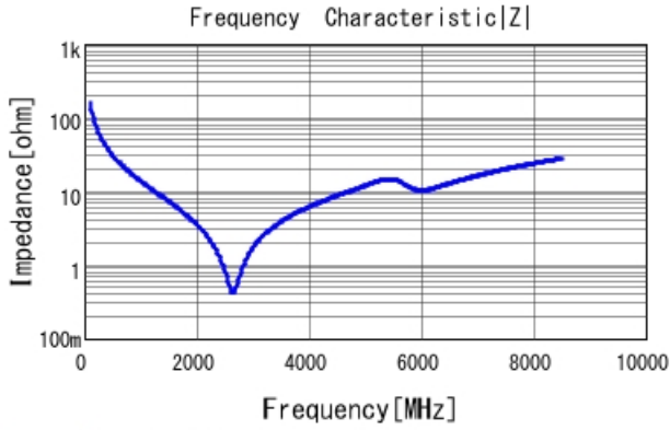
GRM1555C1H100GA01 |Z| DCOV, 25degC
