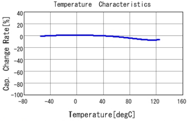
GCM188R71E683KA57 C-Temp. capchange, DC0.0V, AC1.C
