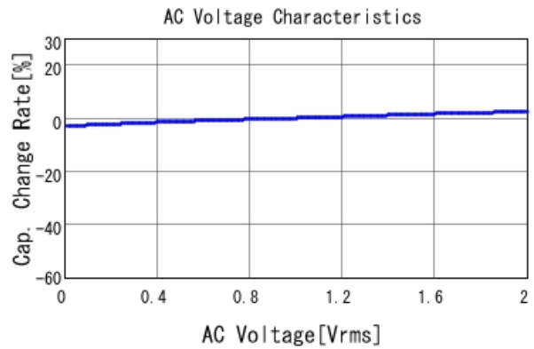
GCM188R71E683KA57 C-AC Voltage capchange, DCOV, 25
