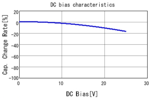
GCM188R71E683KA57 C-DC bias capchange, 25.0degC, A
