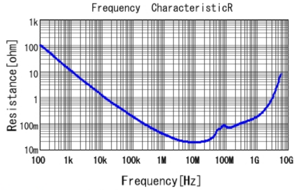
GCM188R71E683KA57 R DCOV, 25degC
