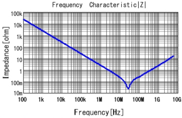
GCM188R71E683KA57 |Z| DCOV, 25degC
