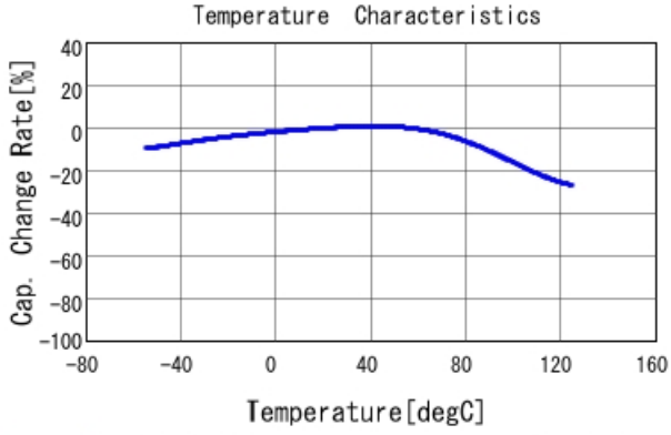
GRM316D71C225KA12 C-Temp. capchange, DC0.0V, AC1.C
