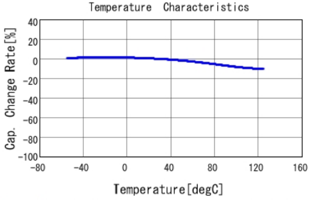
GRM188R71A334KA61 C-Temp. capchange, DC0.0V, AC1.C
