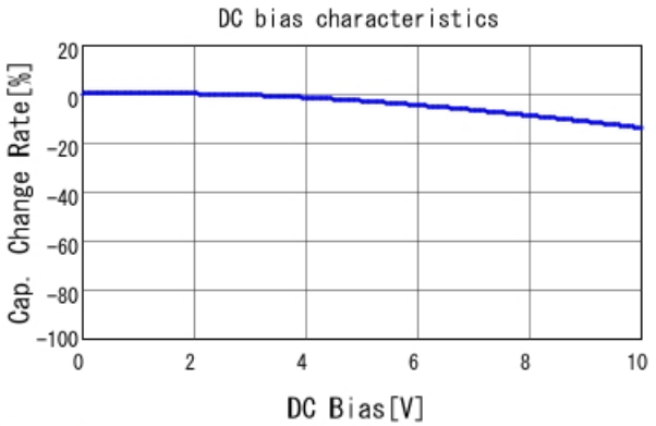
GRM188R71A334KA61 C-DC bias capchange, 25.0degC, A
