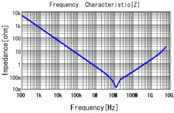
GRM188R71A334KA61 |Z| DCOV, 25degC
