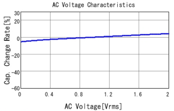
GRM188R71A334KA61 C-AC Voltage capchange, DCOV, 25
