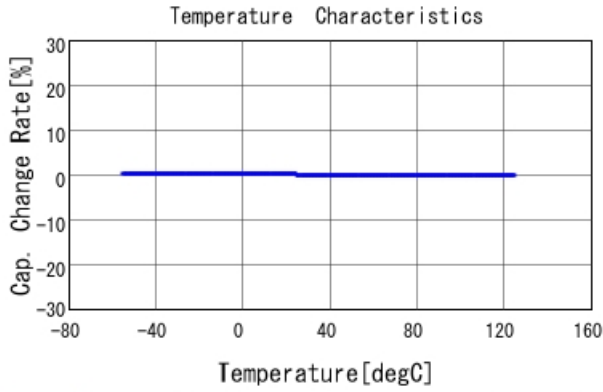
GRM0335C1H4R6BA01 C-Temp. capchange, DCOV, AC1Vrms
