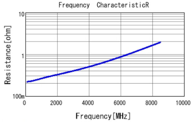
GRM0335C1H4R6BA01 R DCOV, 25degC
