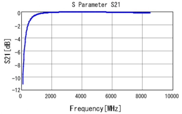
GRM0335C1H4R6BA01 S21 DCOV, 25degC
