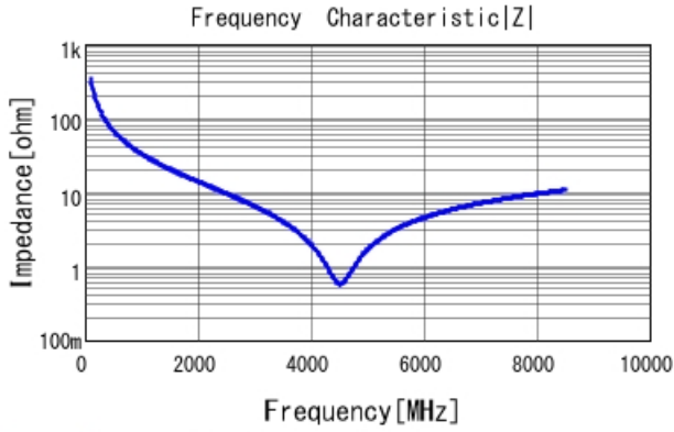
GRM0335C1H4R6BA01 |Z| DCOV, 25degC
