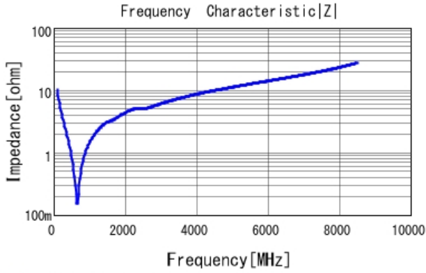
■ GRT1555C1H151JA02 |Z| DC0V, 25degC
