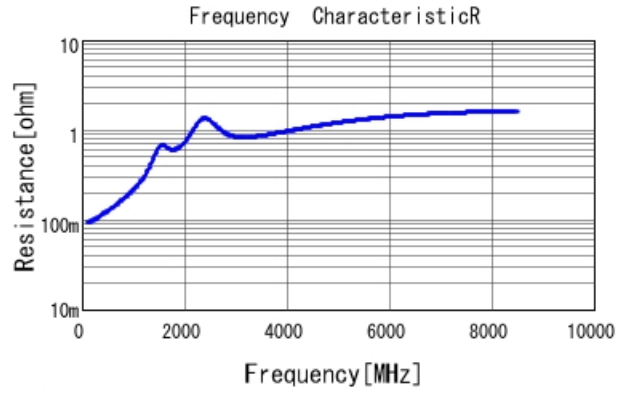
■ GRT1555C1H151JA02 R DC0V, 25degC
