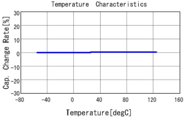
GRM0225C1E7R0BA03 C-Temp. capchange, DCOV, AC1Vrms
