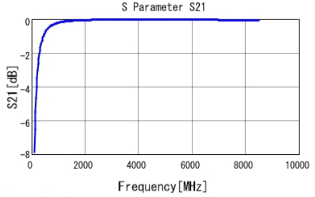
GRM0225C1E7R0BA03 S21 DCOV, 25degC
