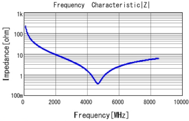
GRM0225C1E7R0BA03 |Z| DCOV, 25degC
