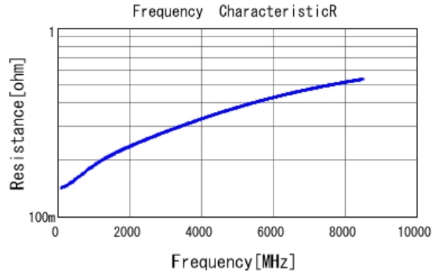
GRM0225C1E7R0BA03 R DCOV, 25degC
