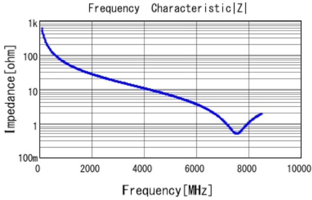
GRM0225C1E2R7WA03 |Z| DCOV, 25degC
