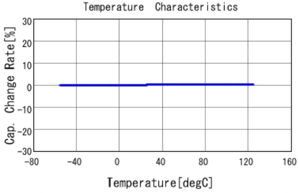
GRM0225C1E2R7WA03 C-Temp. capchange, DCOV, AC1Vrms
