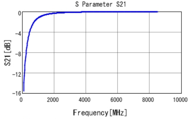
GRM0225C1E2R7WA03 S21 DCOV, 25degC
