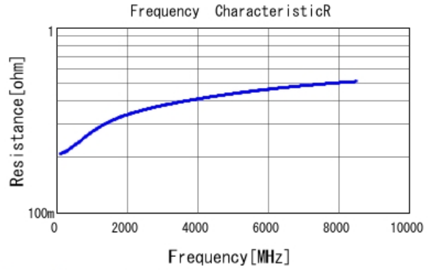
GRM0225C1E2R7WA03 R DCOV, 25degC
