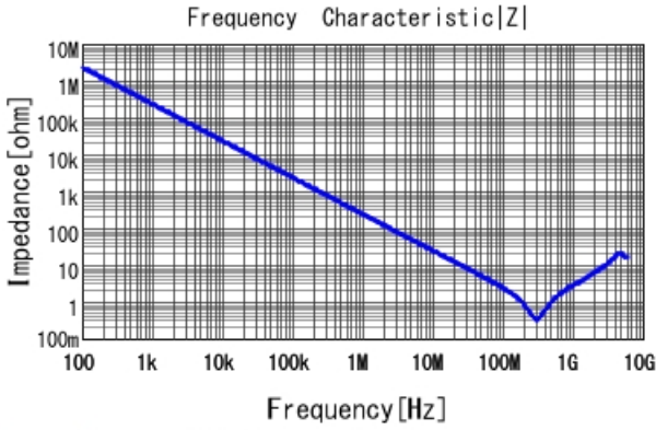
GRM188B11H681KA01 |Z| DCOV, 20degC
