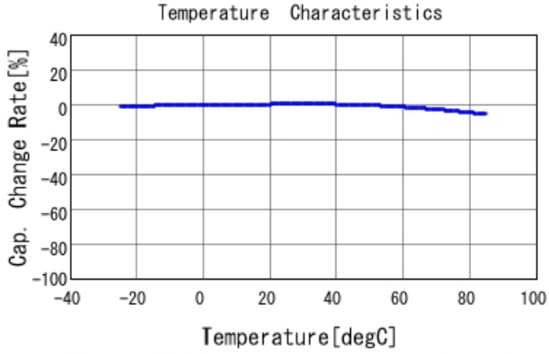
GRM188B11H681KA01 C-Temp. capchange, DC0.0V, AC1.C
