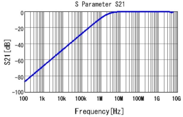
GRM188B11H681KA01 S21 DC0V, 20degC
