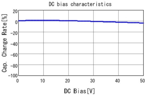
GRM188B11H681KA01 C-DC bias capchange, 20.0degC, A
