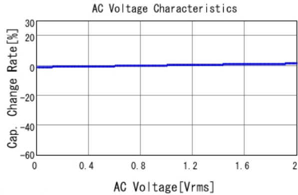
GRM188B11H681KA01 C-AC Voltage capchange, DCOV, 2C
