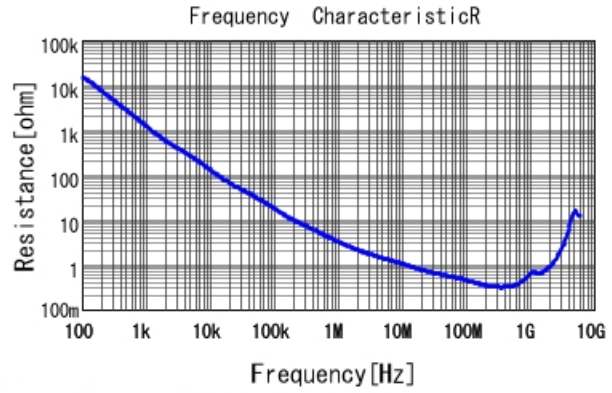
GRM188B11H681KA01 R DCOV, 20degC
