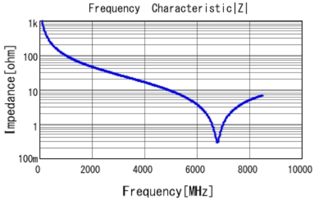
GJM1555C1H1R6WB01 |Z| DCOV, 25degC
