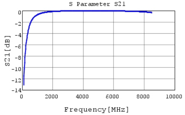
GCQ1555C1H3R6WB01 S21 DCOV, 25degC
