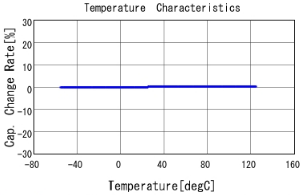
GJM1555C1H6R8CB01 C-Temp. capchange, DCOV, AC1Vrms
