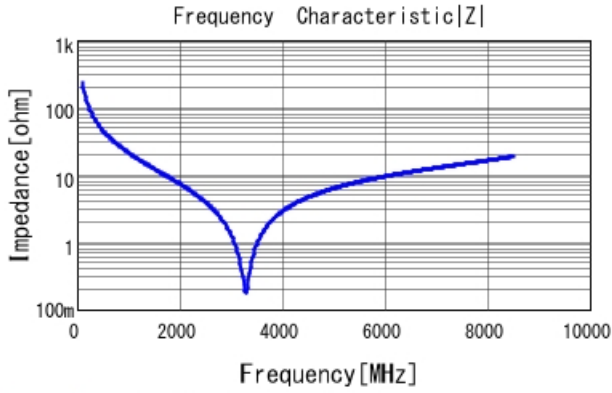
GJM1555C1H6R8CB01 |Z| DCOV, 25degC
