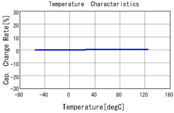
GJM1555C1H5R9BB01 C-Temp. capchange, DC0V, AC1Vrms
