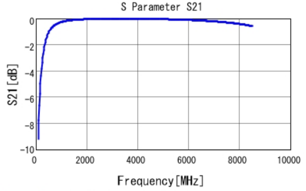
GJM1555C1H5R9BB01 S21 DC0V, 25degC
