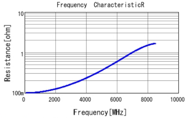
GJM1555C1H5R9BB01 R DCOV, 25degC
