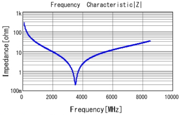
GJM1555C1H5R9BB01 |Z| DCOV, 25degC
