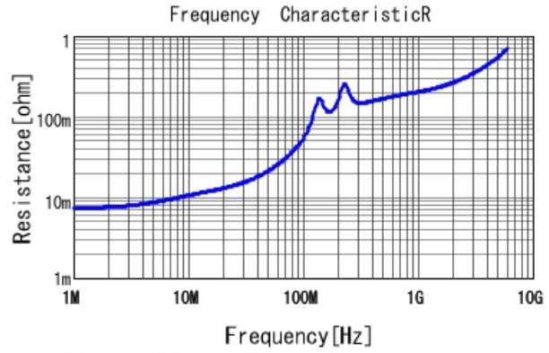
GRM2167U1H153JA01 R DCOV, 25degC
