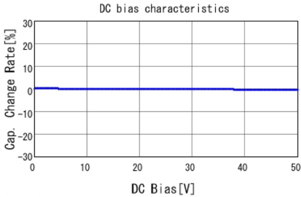
GRM2167U1H153JA01 C-DC bias capchange, 25.0degC, A
