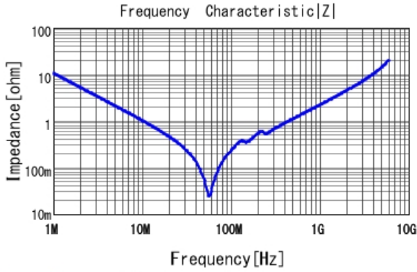
GRM2167U1H153JA01 |Z| DCOV, 25degC
