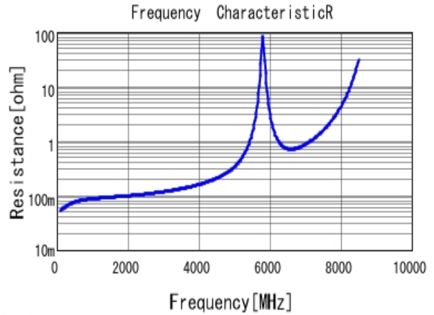
■ GQM2195C2A6R2CB01 R DC0V, 25degC
