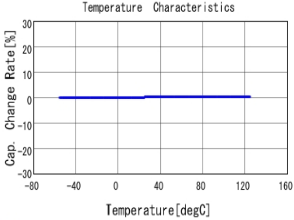
■ GQM2195C2A6R2CB01 C-Temp. capchange, DCOV, AC1Vrms
