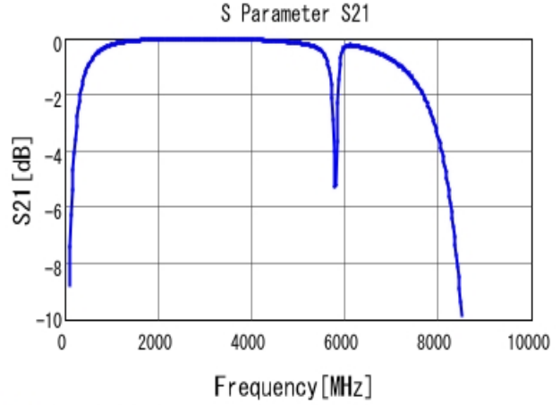
■ GQM2195C2A6R2CB01 S21 DCOV, 25degC
