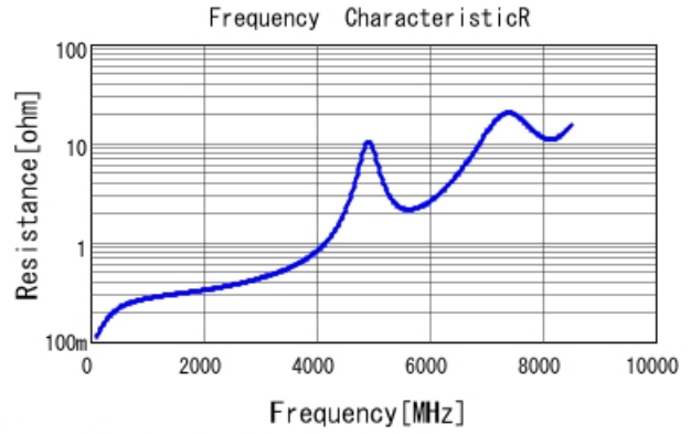
GRM1885C1H8R9BA01 R DCOV, 25degC
