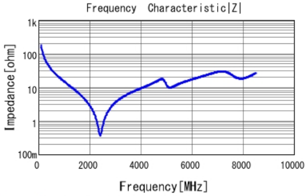
GRM1885C1H8R9BA01 |Z| DCOV, 25degC
