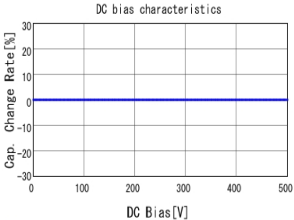
■ GQM22M5C2H1R3BB01 C-DC bias capchange, 25.0degC, AC1V
