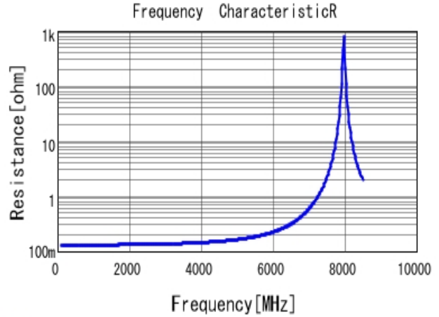
■ GQM22M5C2H1R3BB01 R DC0V, 25degC
