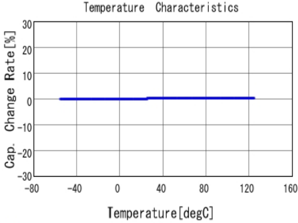
■ GQM22M5C2H1R3BB01 C-Temp. capchange, DCOV, AC1Vrms
