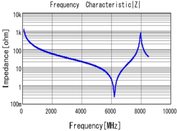
■ GQM22M5C2H1R3BB01 |Z| DC0V, 25degC
