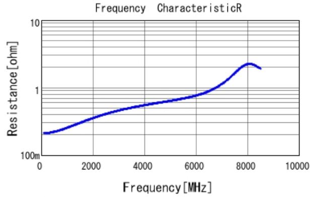
GRM1555C2A4R9BA01 R DCOV, 25degC
