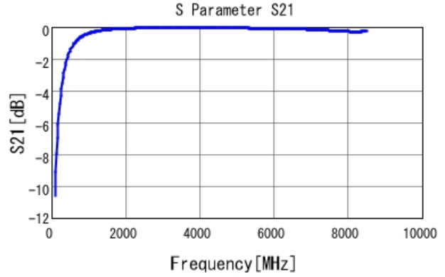
GRM1555C2A4R9BA01 S21 DC0V, 25degC
