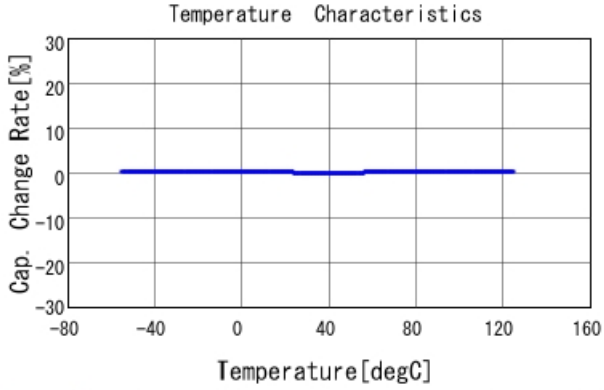
GRM1555C2A4R9BA01 C-Temp. capchange, DC0V, AC1Vrms
