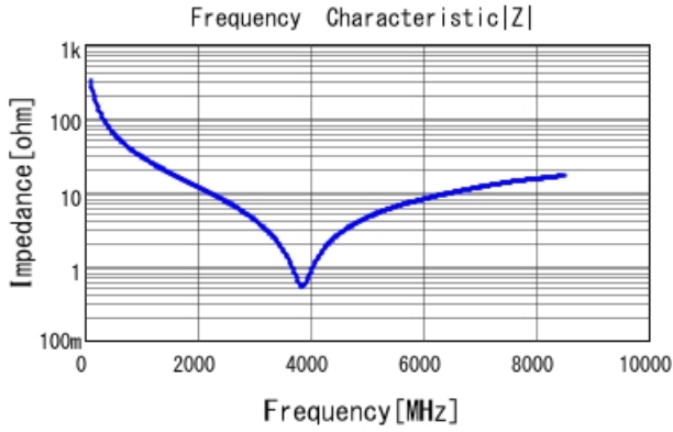
GRM1555C2A4R9BA01 |Z| DCOV, 25degC
