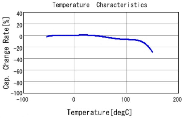
GCJ31CL8YA564KA01 C-Temp. capchange, DC0.0V, AC1.C
