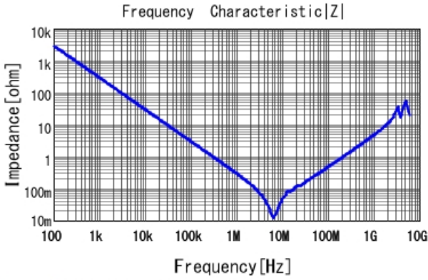
GCJ31CL8YA564KA01 |Z| DCOV, 25degC
