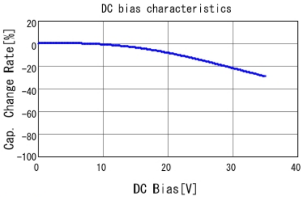
GCJ31CL8YA564KA01 C-DC bias capchange, 25.0degC, A
