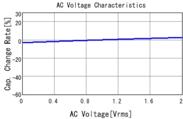
GCJ31CL8YA564KA01 C-AC Voltage capchange, DCOV, 25
