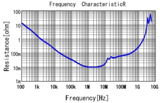
GCJ31CL8YA564KA01 R DCOV, 25degC
