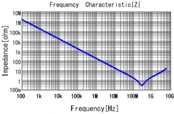
GCM155L81H102KA37 |Z| DCOV, 25degC
