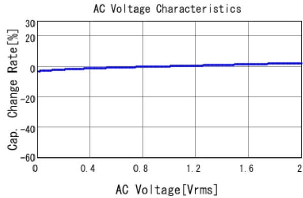
GCM155L81H102KA37 C-AC Voltage capchange, DCOV, 25
