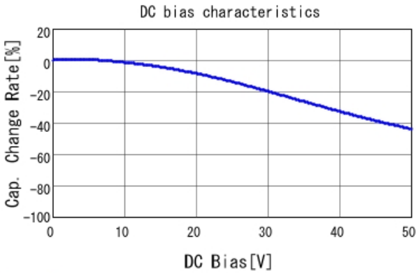
GCM155L81H102KA37 C-DC bias capchange, 25.0degC, A
