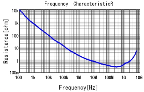
GCM155L81H102KA37 R DCOV, 25degC
