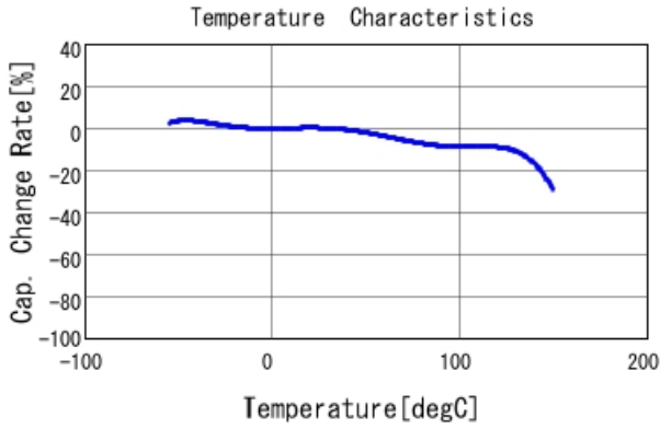
GCM155L81H102KA37 C-Temp. capchange, DC0.0V, AC1.C
