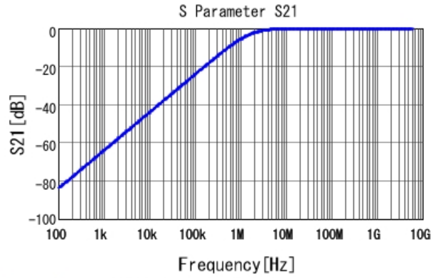
GCM155L81H102KA37 S21 DC0V, 25degC
