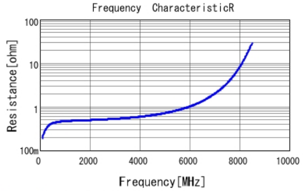
GRM1885C1H3R4WA01 R DCOV, 25degC
