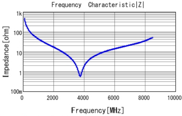
GRM1885C1H3R4WA01 |Z| DCOV, 25degC
