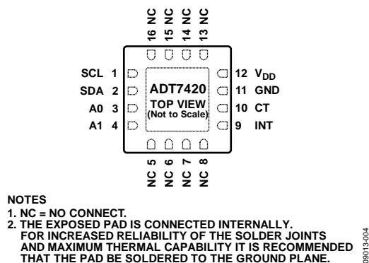
Figure 3. Pin Configuration
