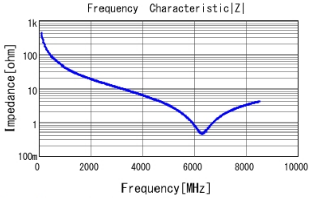
GRM0225C1E3R8CA03 |Z| DCOV, 25degC
