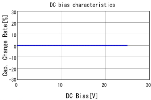
GRM0225C1E3R8CA03 C-DC bias capchange, 25.0degC, A
