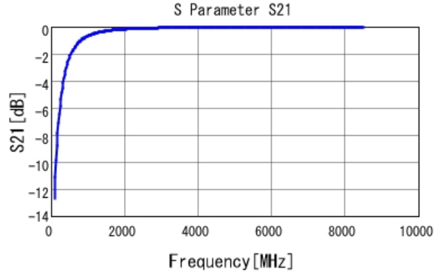
GRM0225C1E3R8CA03 S21 DC0V, 25degC
