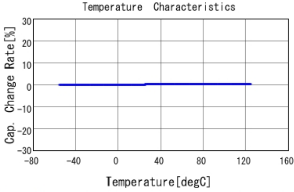
GRM0225C1E3R8CA03 C-Temp. capchange, DC0V, AC1Vrms
