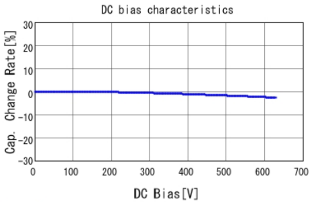
GRM32D7U2J822JW31 C-DC bias capchange, 25.0degC, A
