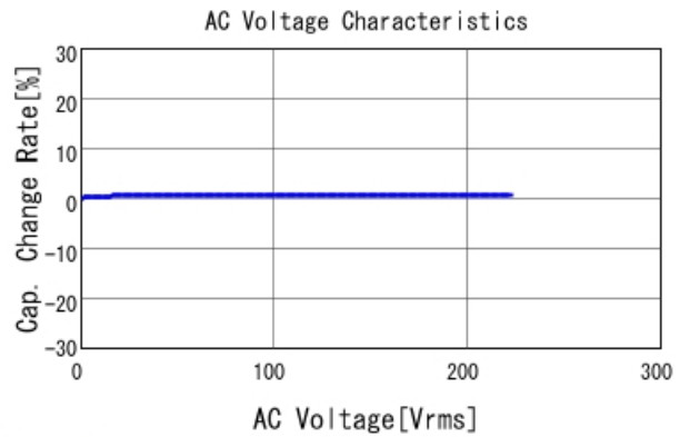
GRM32D7U2J822JW31 C-AC Voltage capchange, DCOV, 25
