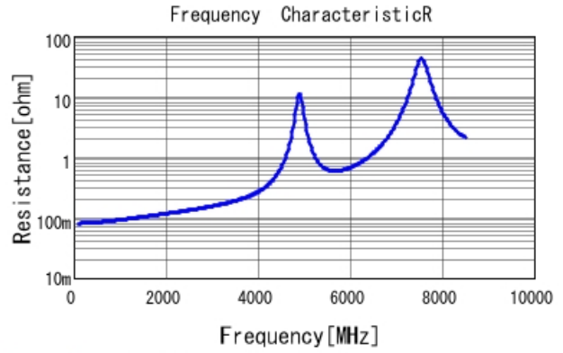
GJM1555C1H180JB01 R DCOV, 25degC
