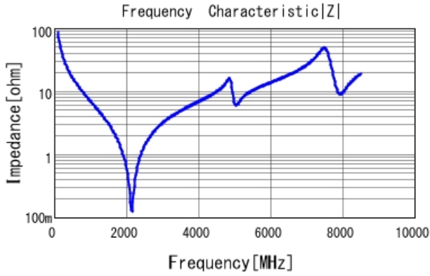
GJM1555C1H180JB01 |Z| DCOV, 25degC
