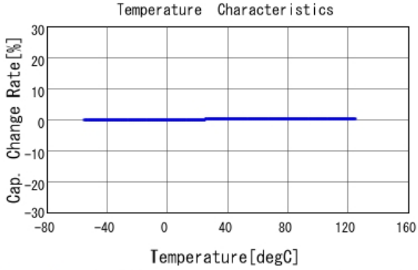
GJM1555C1H180JB01 C-Temp. capchange, DCOV, AC1Vrms
