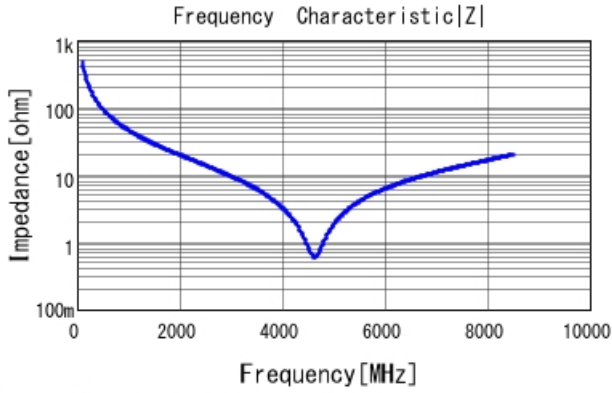
GRM1555C1H3R3BA01 |Z| DCOV, 25degC
