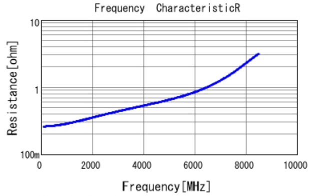
GRM1555C1H3R3BA01 R DCOV, 25degC
